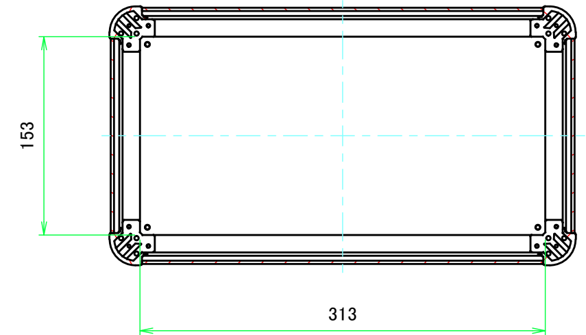
C-C (1:4)
